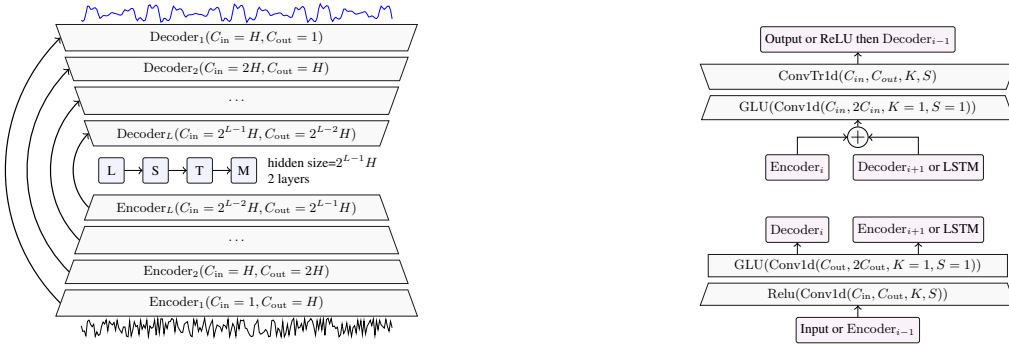
(a) Causal DEMUCS with the noisy speech as input on the bottom and the clean speech as output on the top. Arrows represents U-Net skip connections. H controls the number of channels in the model and L its depth.
