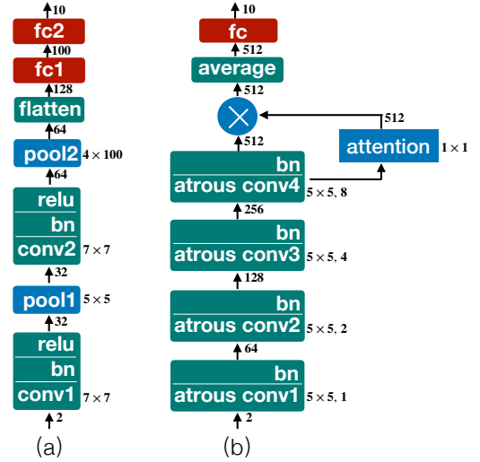
Figure 1: Acoustic scene classifiers used in this work: (a) Baseline model of DCASE2019. Kernel size for each convolutional layer is labelled besides the block, and the number of channels is denoted between each block transition. (b) Attentive atrous CNN. Dilation size for each atrous convolutional layer is given next to the kernel size.
