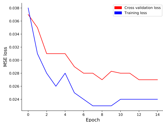
Figure 3: MSE loss for REVERB challenge dataset
