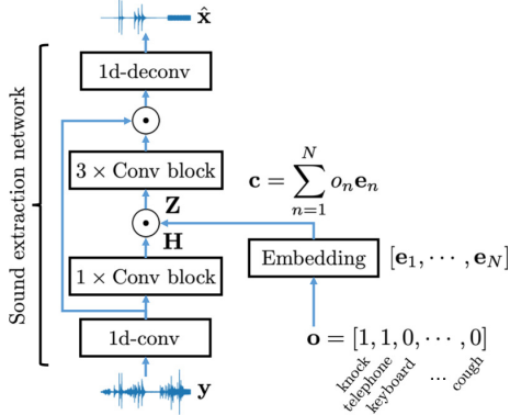
Figure 1: Overview of proposed Sound Selector architecture.
