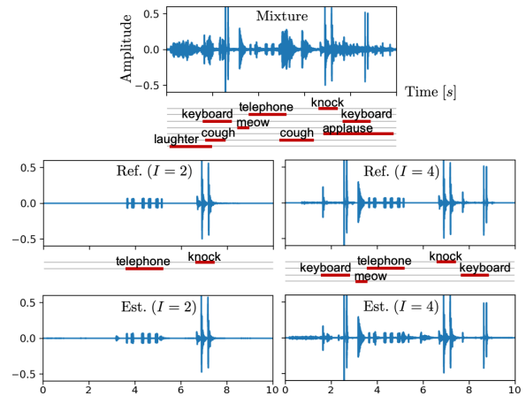
Figure 2: Mixture with AEs from 7 AE classes, the reference signals (Ref.), and the signals estimated with the proposed Sound Selector (Est.) for 2 (left) and 4 (right) target AE classes.
