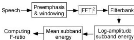
Figure 3. Procedure to obtain the mean subband energy.
