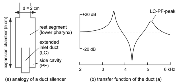
Figure 2. Model geometry and acoustic simulation. (a) Duct model of the lower vocal tract and (b) Result of duct model simulation showing a peak-dip-peak transfer function.
